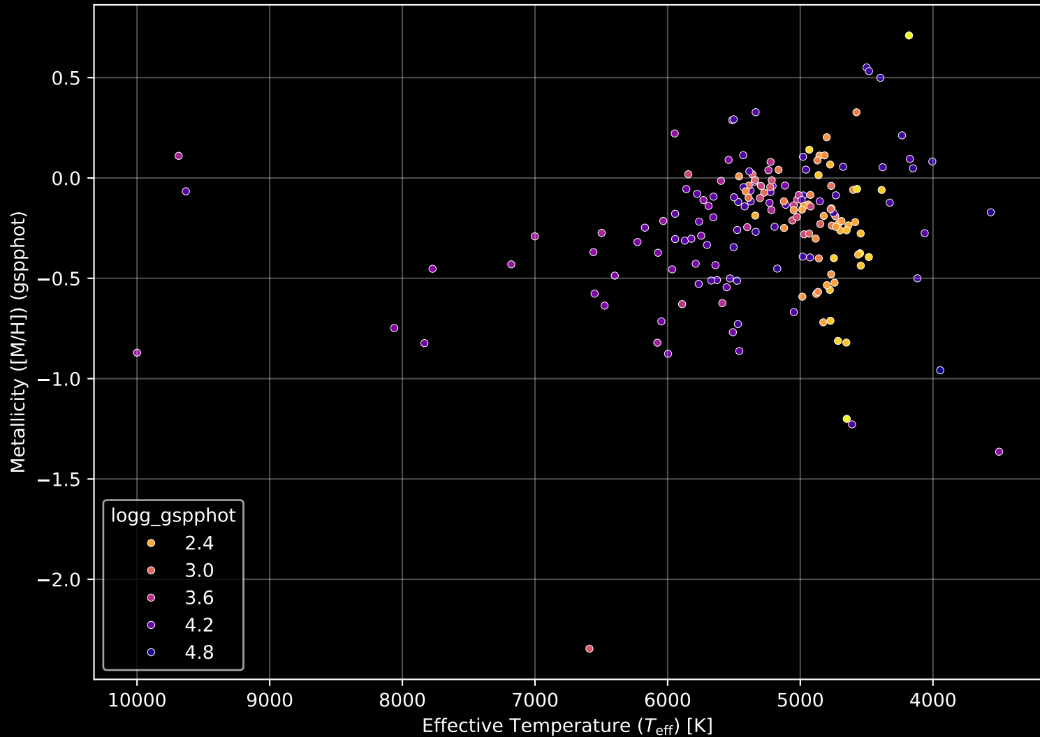
APOGEE DR17 Field: [167+31_MGA] Stellar Population Parameters (n= 178)
