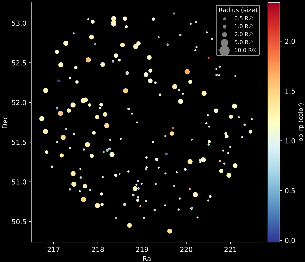
APOGEE DR17 Field: [167+31_MGA] Stars: 178
