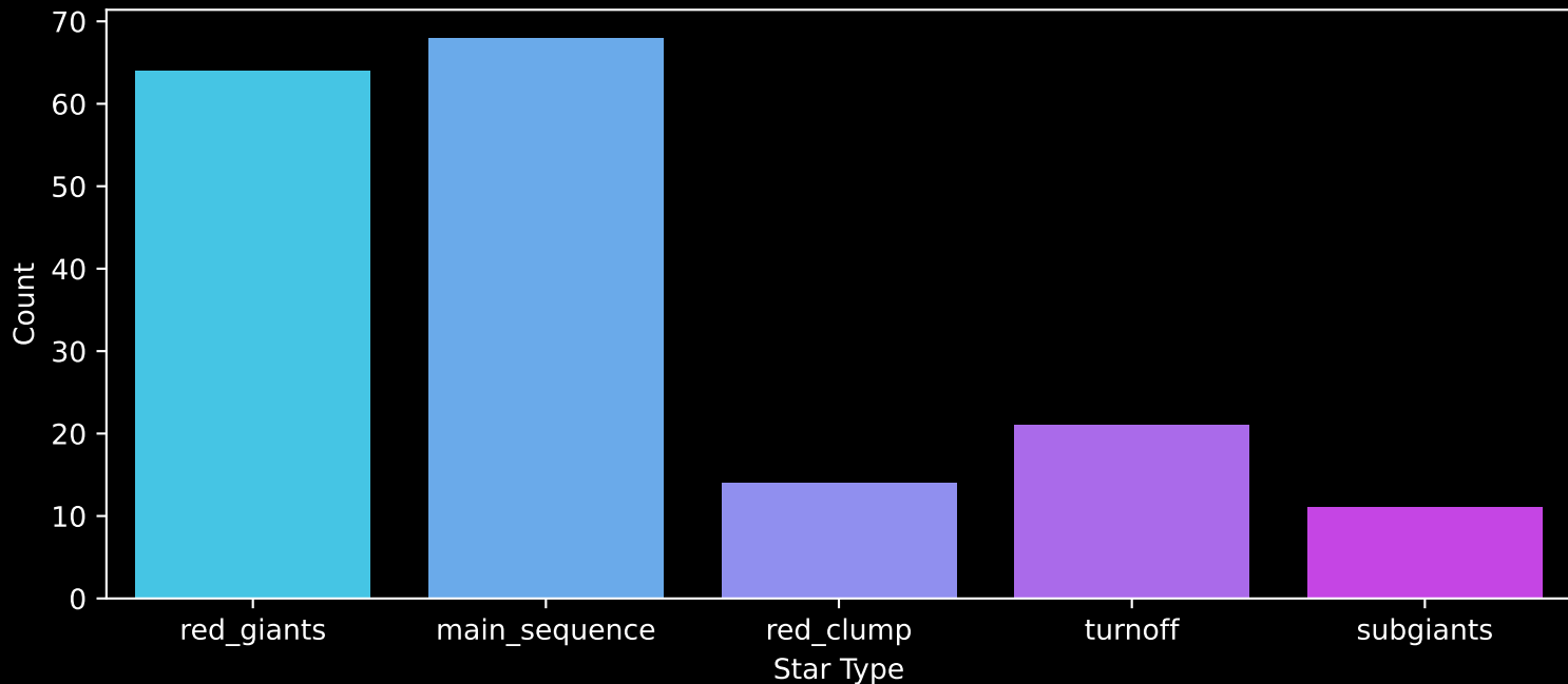
APOGEE DR17 Field: [167+31_MGA] Count plot of Star Type
