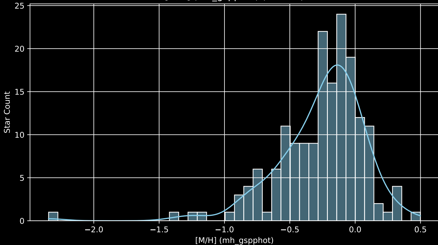
APOGEE DR17 Field: [167+31_MGA [M/H] (mh_gspphot) (n= 175)
