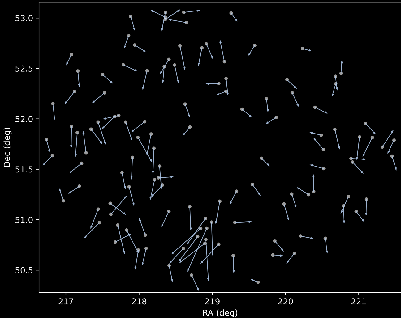
APOGEE DR17 Cluster 1 Proper Motion Vectors (n=119)
