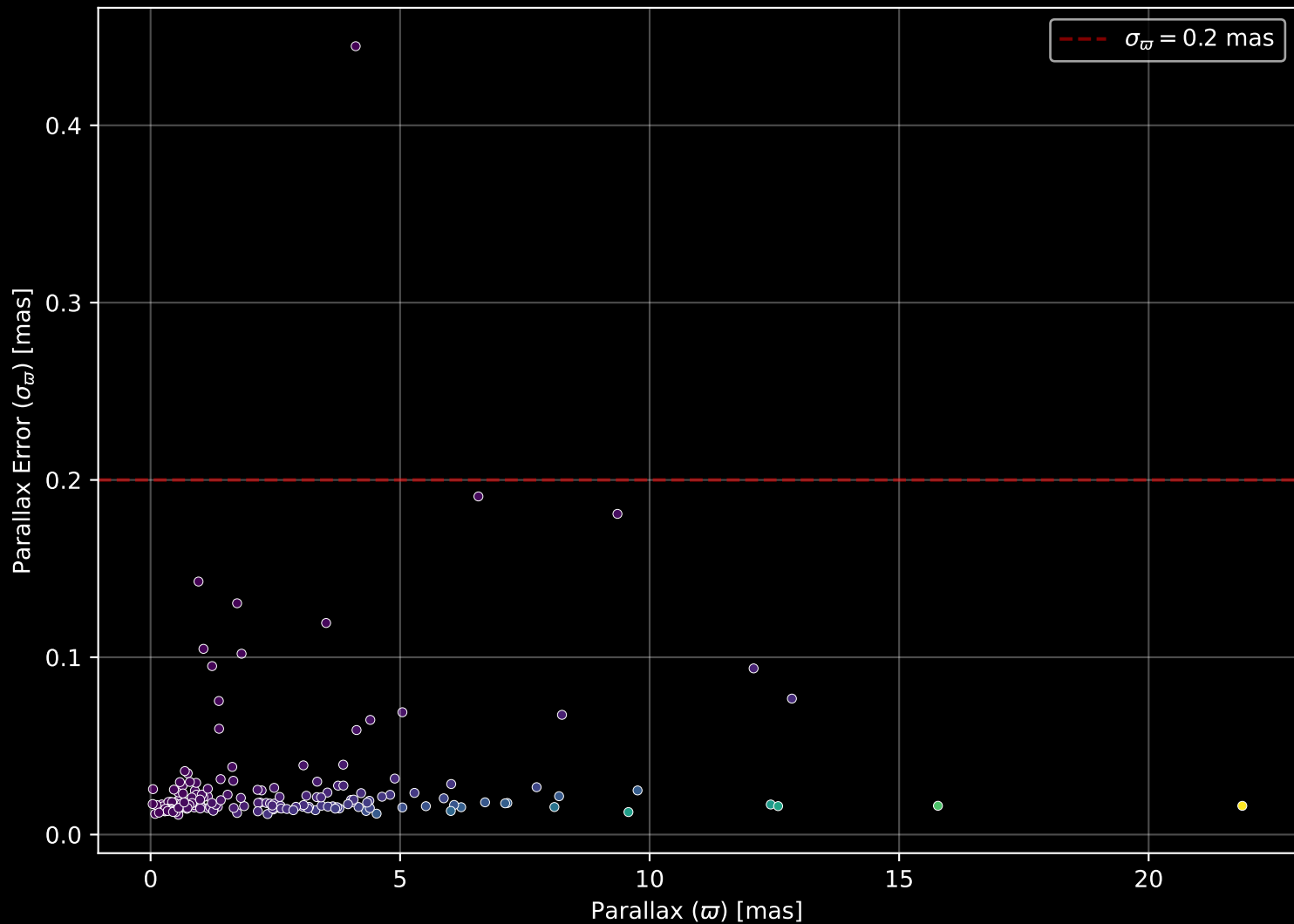
APOGEE DR17 Field: [167+31_MGA] Parallax Quality (n= 178)
