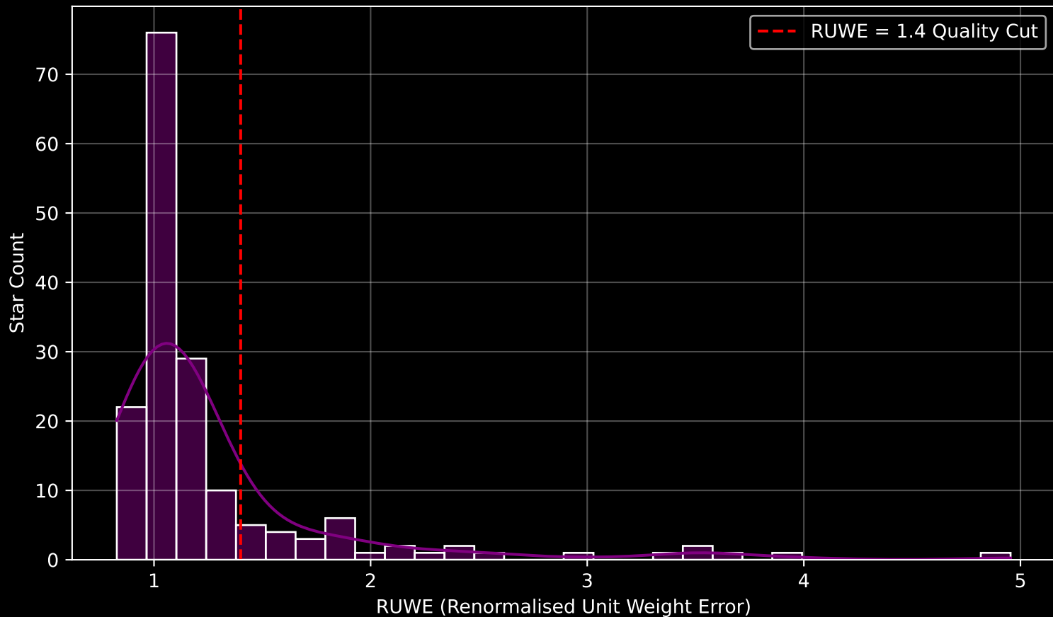
GAPOGEE DR17 Field [167+31_MGA] RUWE Distribution (n= 169)
