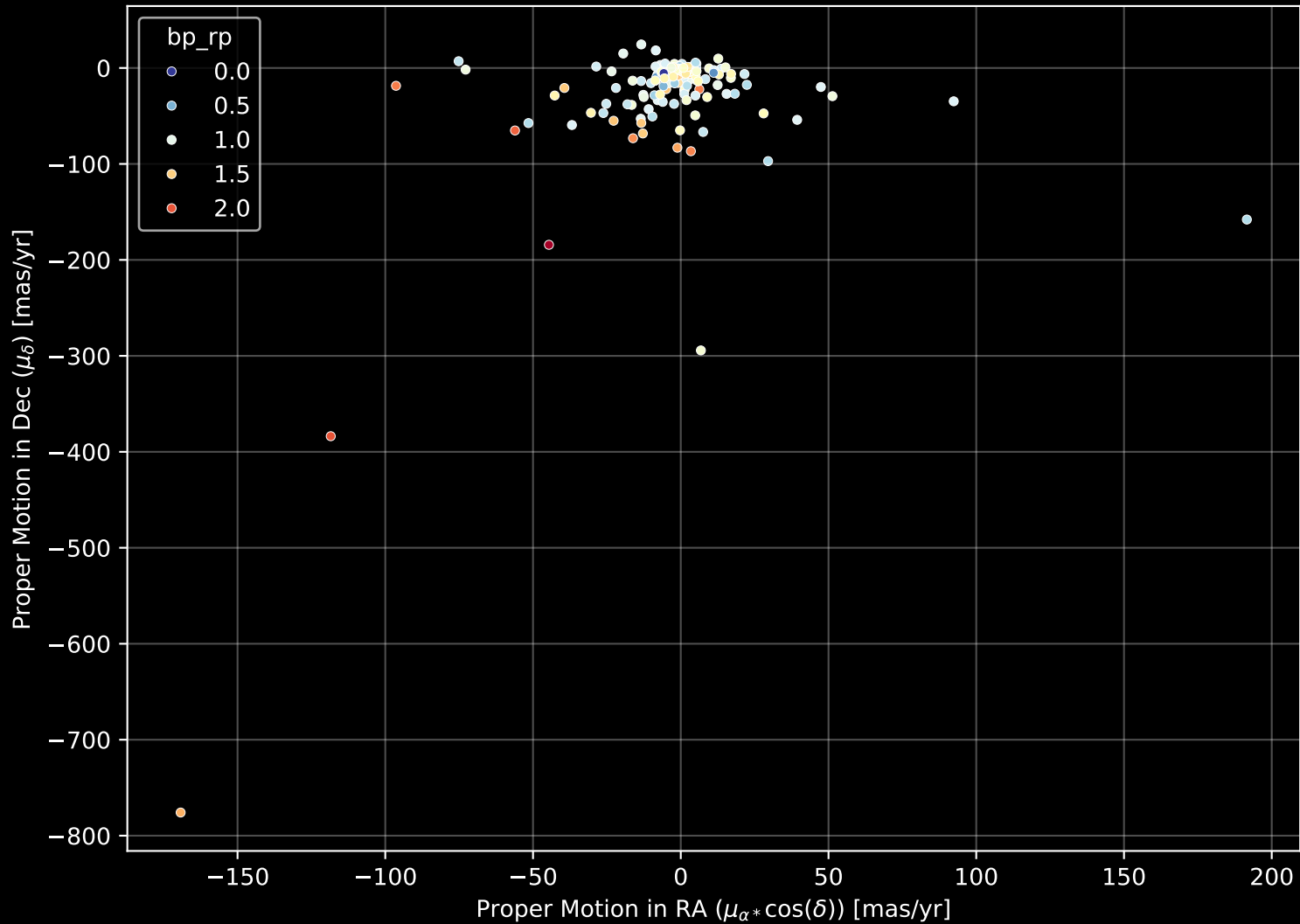
APOGEE DR17 Field: [167+31_MGA] Proper Motion Diagram (n= 178)
